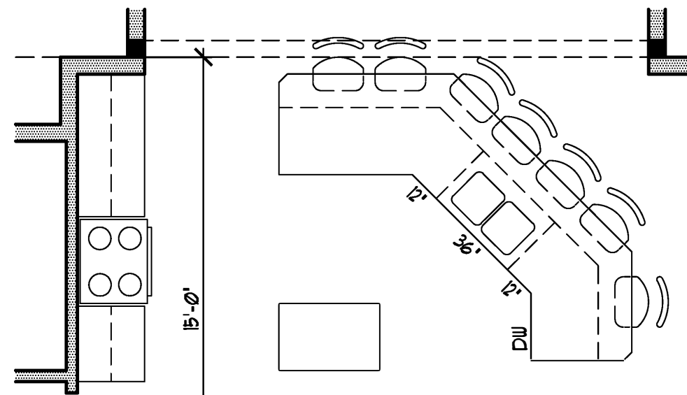
OPT. KITCHEN PLAN
